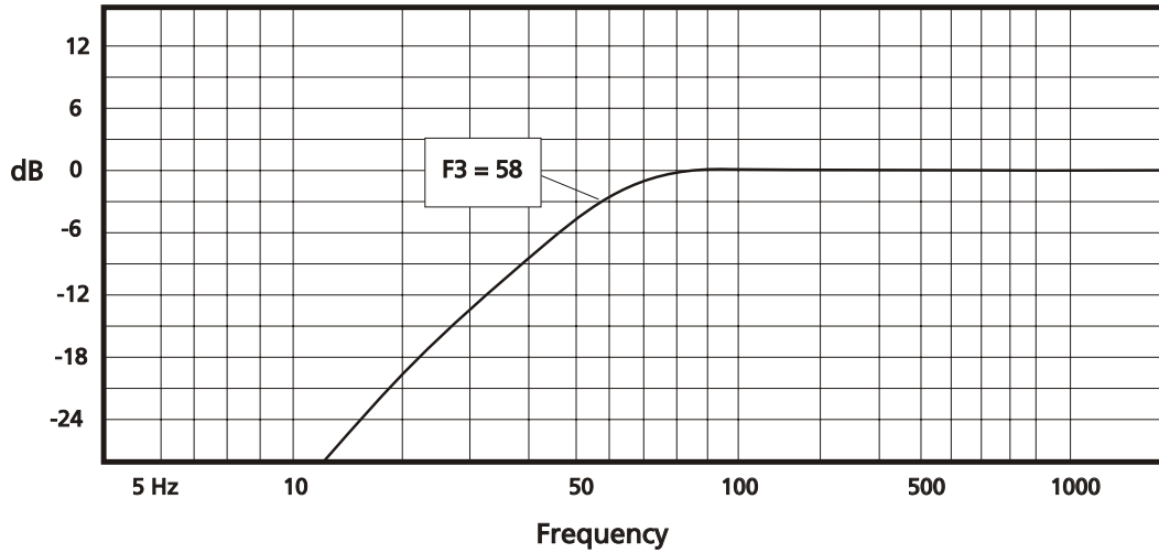
EL1008 Amplitude Response (dB/Hz)
