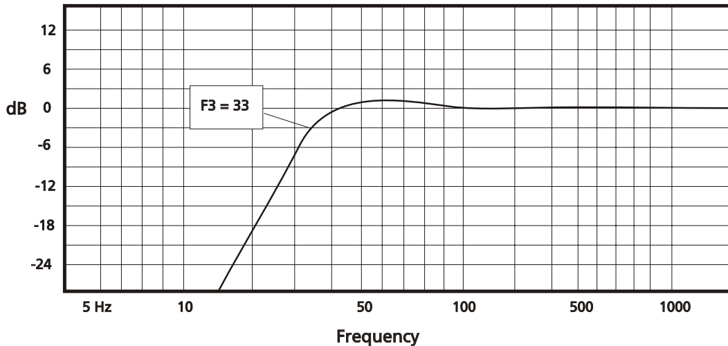
EL1008 Amplitude Response (dB/Hz)
