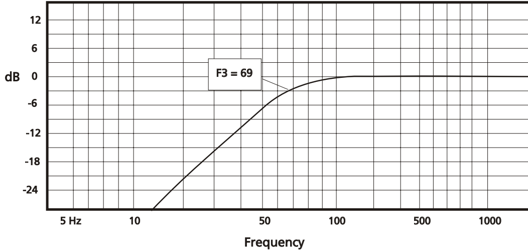
EL1204 Amplitude Response (dB/Hz)
