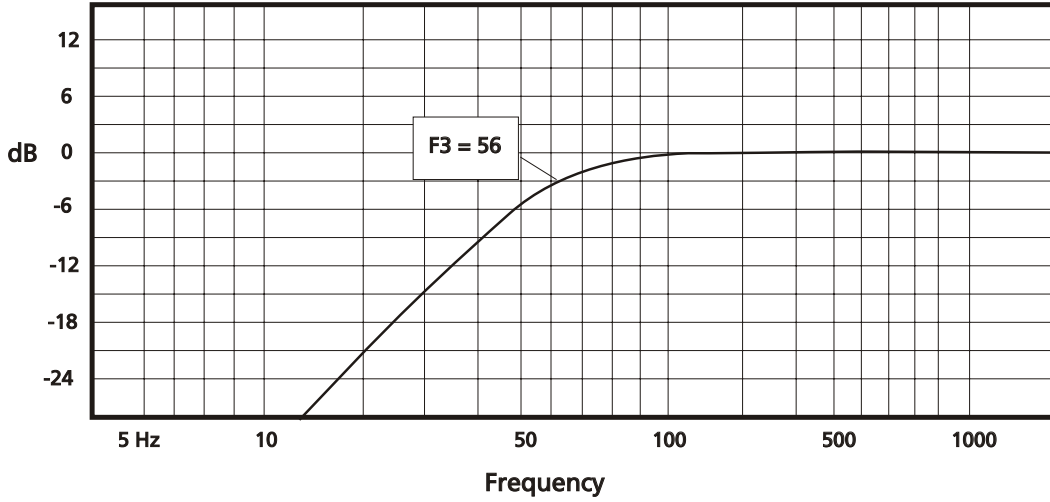
EL1208 Amplitude Response (dB/Hz)
