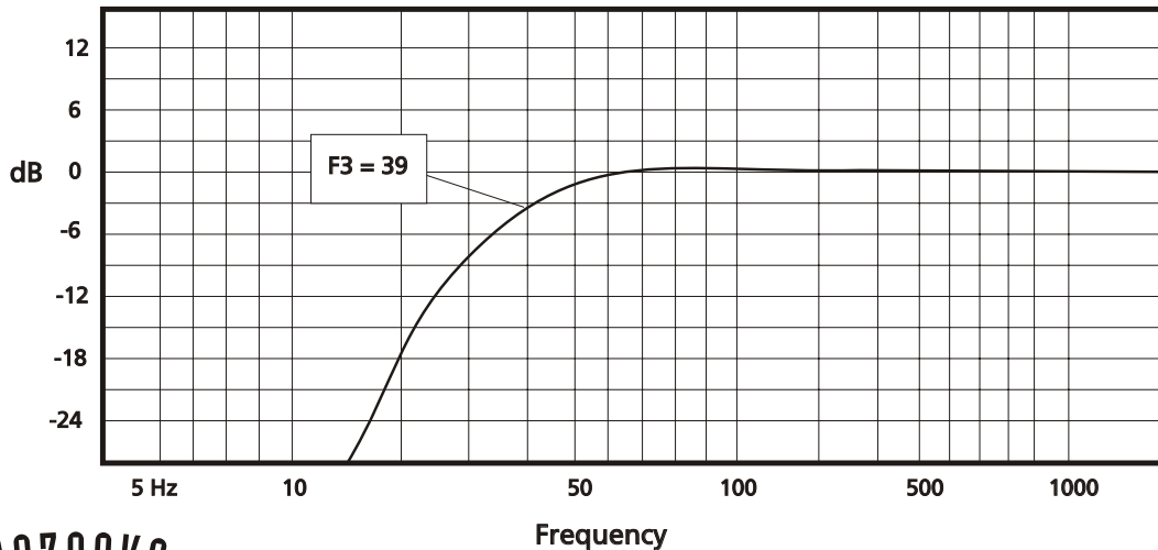
EL1204 Amplitude Response (dB/Hz)
