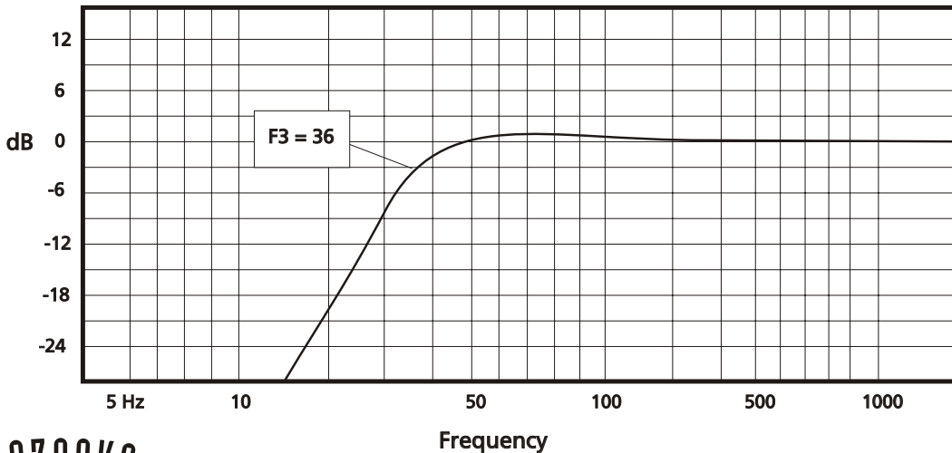
EL1208 Amplitude Response (dB/Hz)
