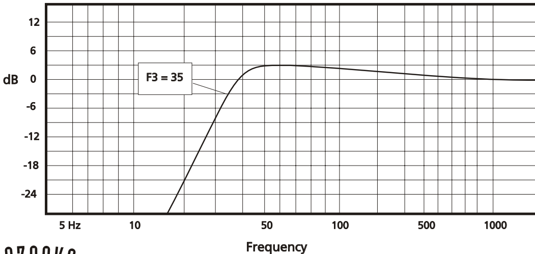
RSW1224DV Amplitude Response (dB/Hz)
