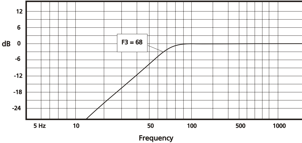
RSW1024DV Amplitude Response (dB/Hz)
