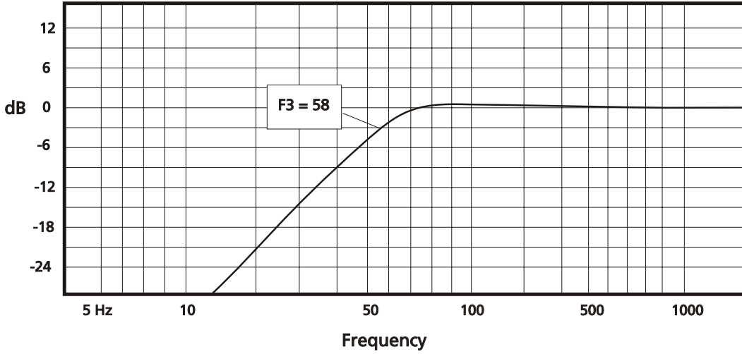
RSW1224DV Amplitude Response (dB/Hz)
