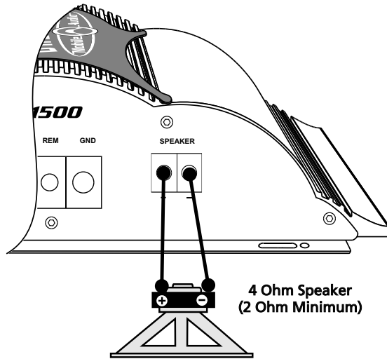
EL1500 SPEAKER CONNECTIONS
