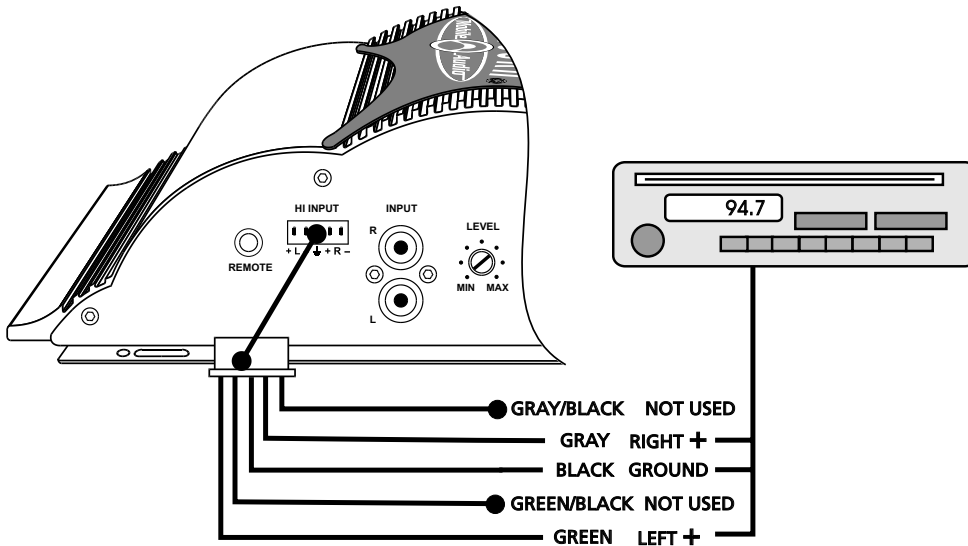
TWO CHANNEL CONNECTIONS: COMMON GROUND RADIO
