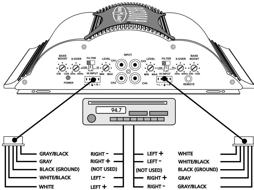
EL460 CONNECTIONS: FLOATING GROUND RADIO (MOST COMMON TYPE)
