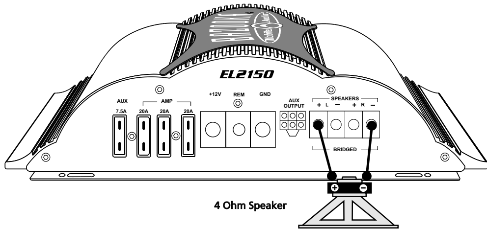
TWO CHANNEL BRIDGED SPEAKER CONNECTIONS
