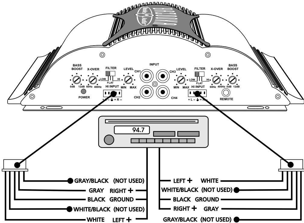
EL460 CONNECTIONS: COMMON GROUND RADIO
