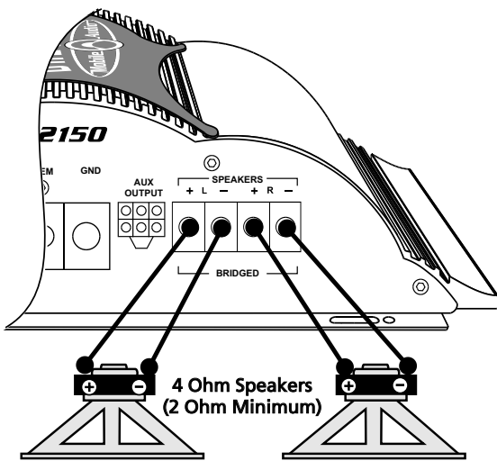
TWO CHANNEL SPEAKER CONNECTIONS
