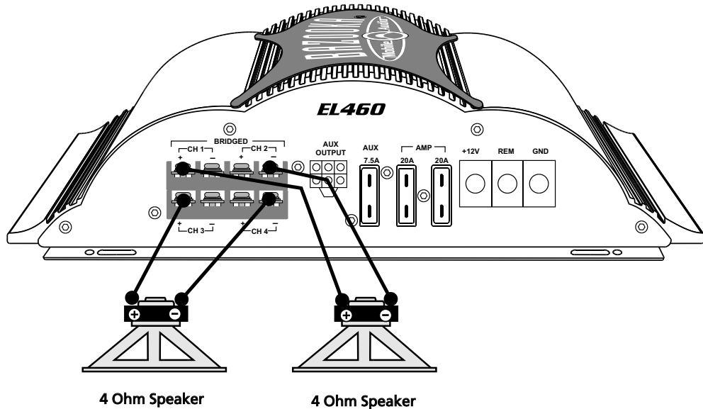
FOUR CHANNEL BRIDGED SPEAKER CONNECTIONS
