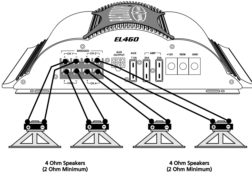
FOUR CHANNEL SPEAKER CONNECTIONS
